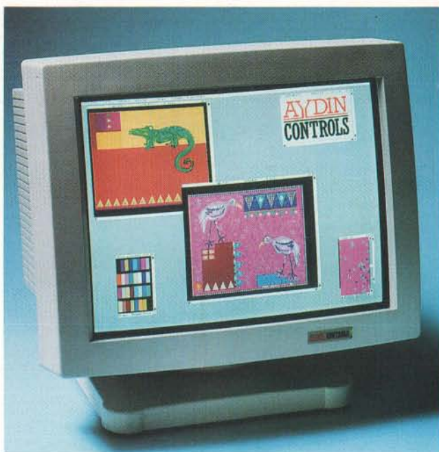
The Ranger 4317 color monitor automatically synchronizes at horizontal frequencies between 30 and 75 kHz and vertical frequencies between 50 and 90 Hz.
